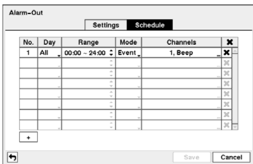
Figure 29 — Alarm-Out Schedule screen.
