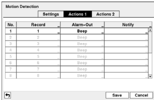
Figure 46 — Motion Detection Actions 1 screen.
