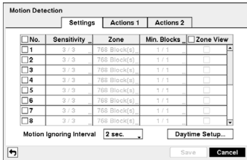
Figure 45 — Motion Detection Settings screen.
